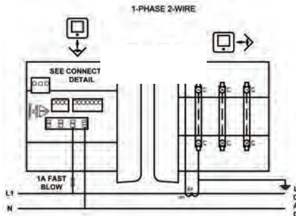
1-phase 2-wire
