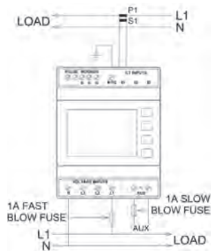
Single-phase, 2-wire
