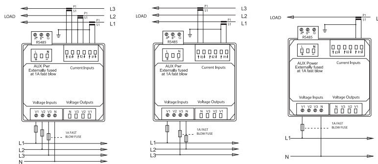
3-phase 4-wire
