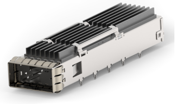
1x1 cage with extruded aluminum heatsinks
